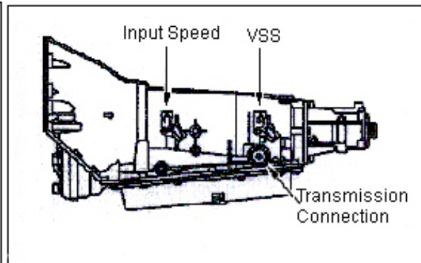
FIGURE 6.23 A/T Input Speed & VSS Sensor, Transmission Connection (4L80E)
