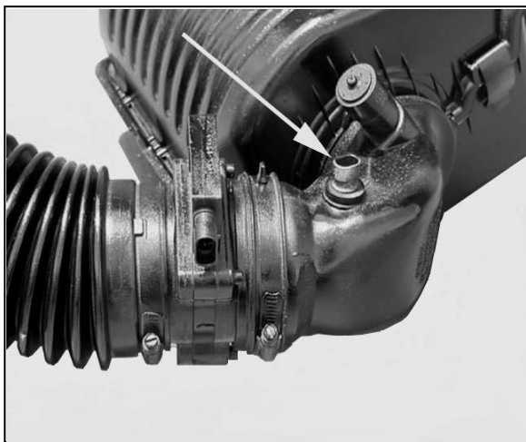
FIGURE 6.20 IAT Sensor
