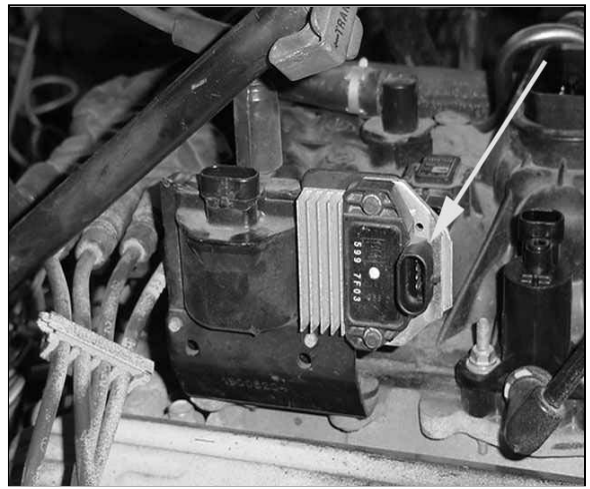
FIGURE 6.13 Coil Driver
