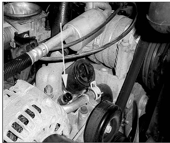
FIGURE 6.19 ECT Sensor
