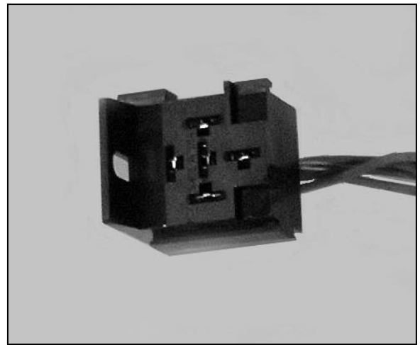
FIGURE 6.5 Fuel Pump Relay Connector
