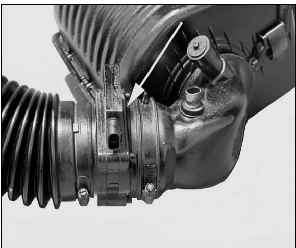
FIGURE 6.16 MAF Sensor
