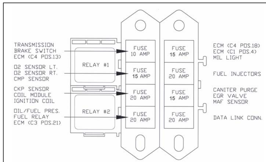
FIGURE 6.26 Fuse Identification
