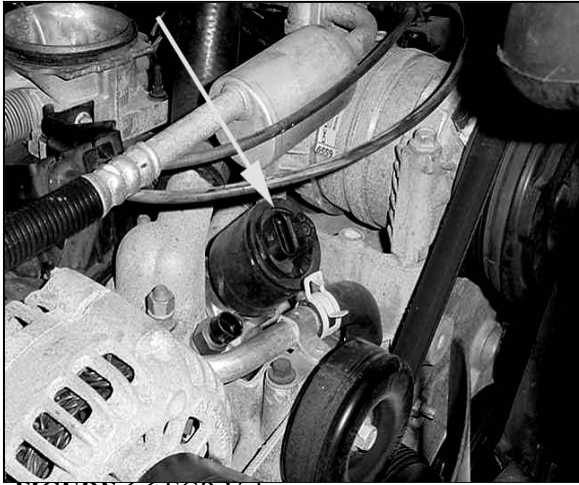
FIGURE 6.6 EGR Valve
