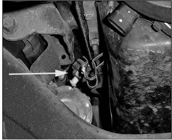
FIGURE 6.7 Knock Sensor Connector
