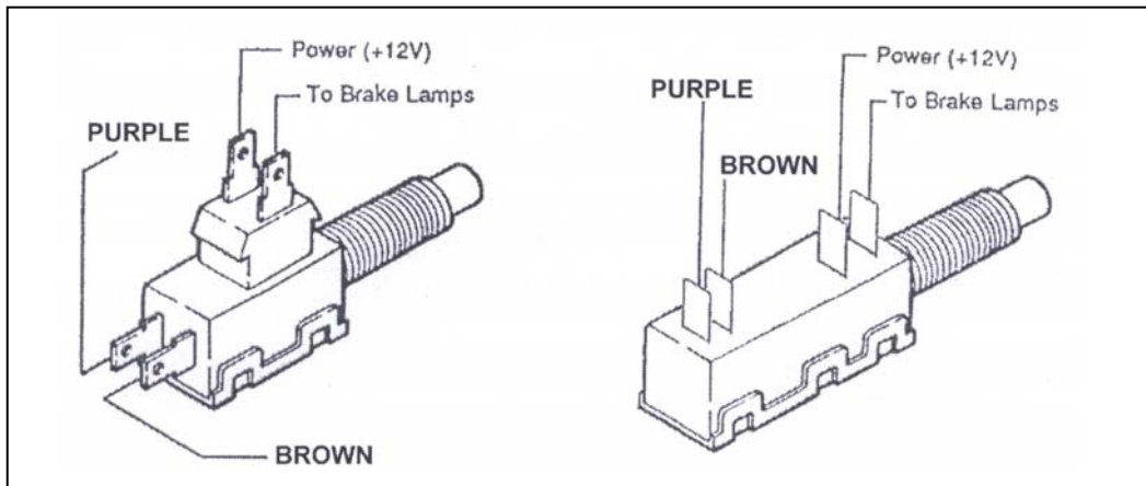
FIGURE 6.2 Brake Switch Connection
