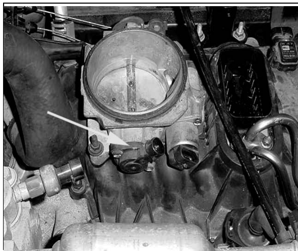
FIGURE 6.14 TPS Sensor
