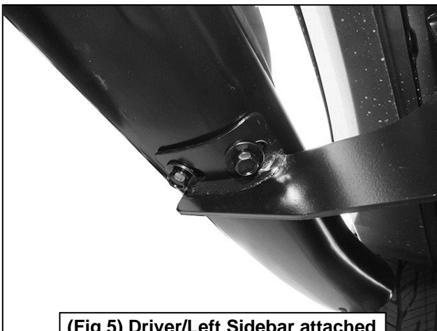
(Fig 5) Driver/Left Sidebar attached to the front Mounting Bracket
