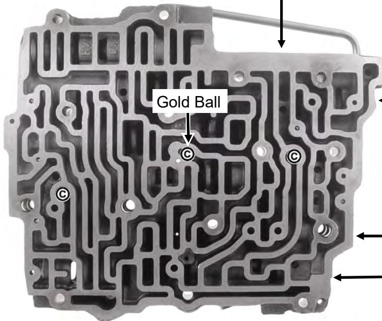
Valve Body Check Ball Locations ©
