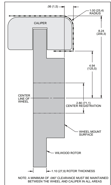
Figure 3B, P/N 140-16132. Wheel Clearance Diagram
