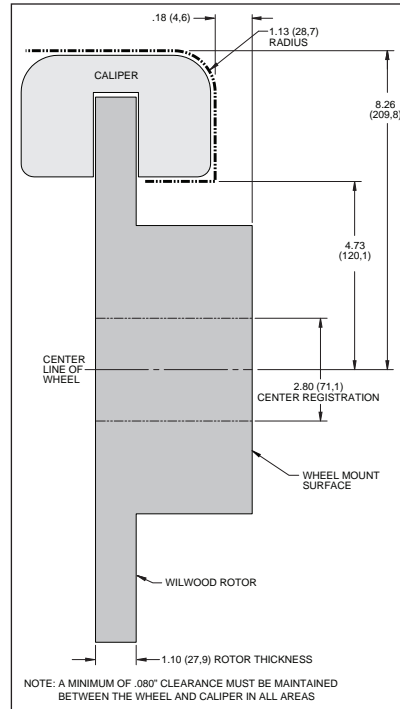
Figure 3A P/N 140-15846. Wheel Clearance Diagram
