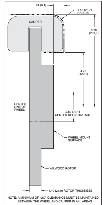
Figure 3B P/N 140-16170. Wheel Clearance Diagram
