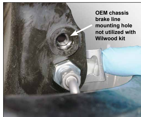
Photo 10 Chassis fitting (TRX model not shown)
