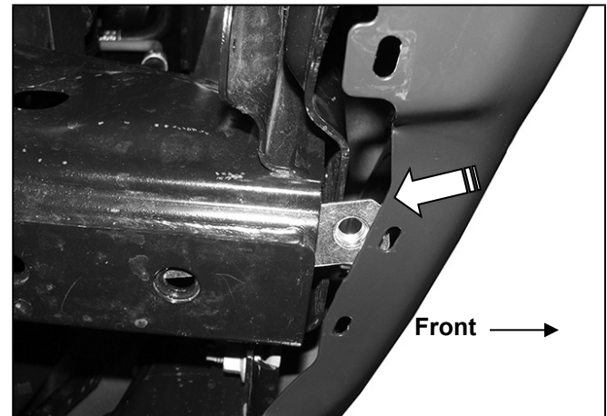
(Fig 4B) Insert Nut Plate into open end of frame- applies to models without tow hooks only
