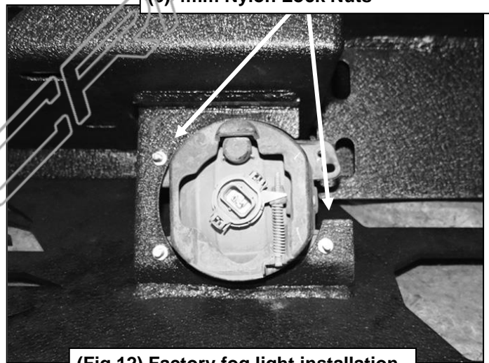
(Fig 12) Factory fog light installation
