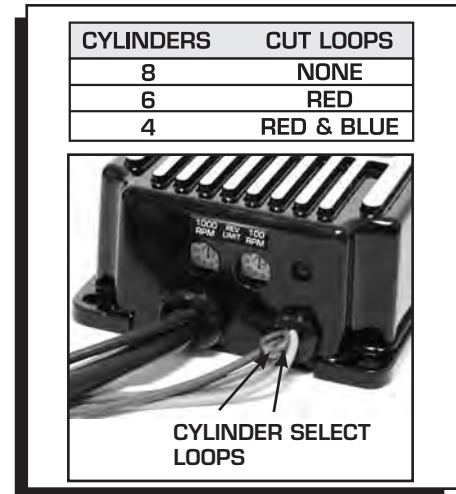
Figure 1 Selecting the number of Cylinders.
