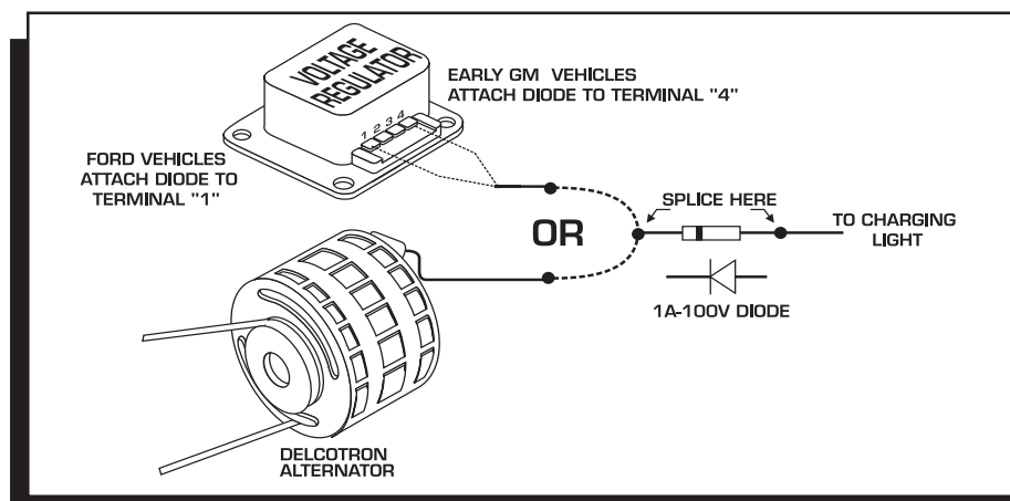
Figure 6 Installing the Diode to fix Run-On.
