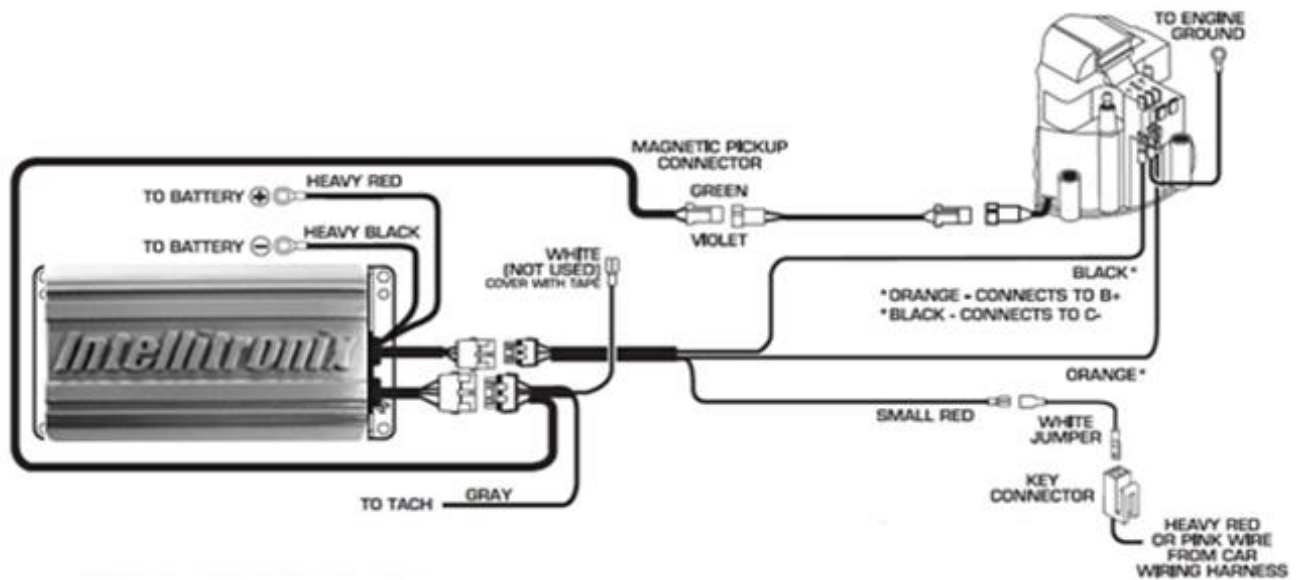
FIG. 6 GM IGNITIONS – WIRING AN HEI 4-PIN MODULE (MAGNETIC PICKUP TRIGGER (continued)
