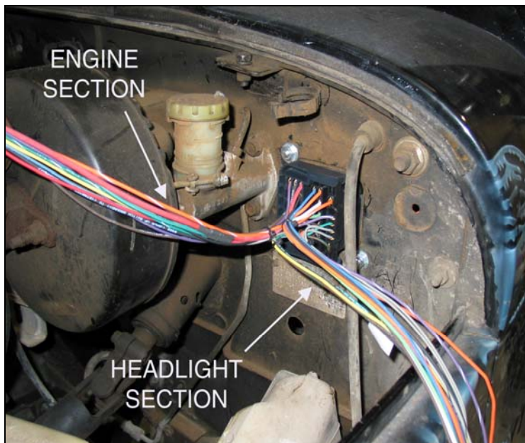
Figure 9.0 Front Harness
