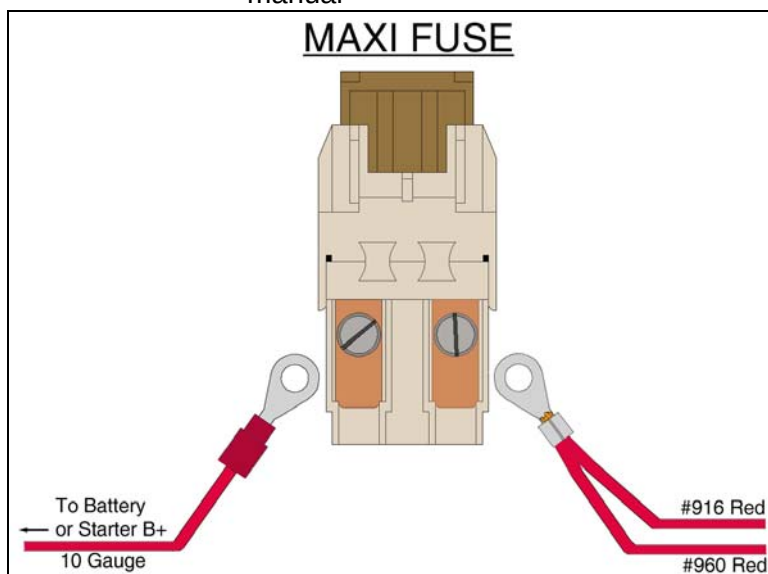
Diagram 8 Maxi Fuse
