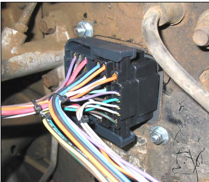
Figure 6.1.3 Bulkhead Mounted
