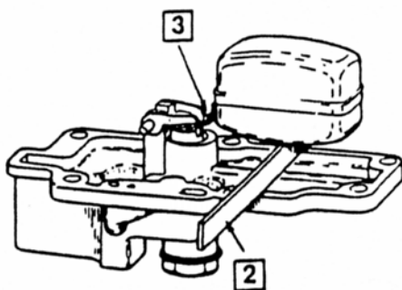
FIG. 2 FLOAT DROP ADJUSTMENT
