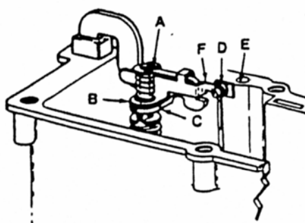
FIG. 3 METERING ROD ADJUSTMENT
