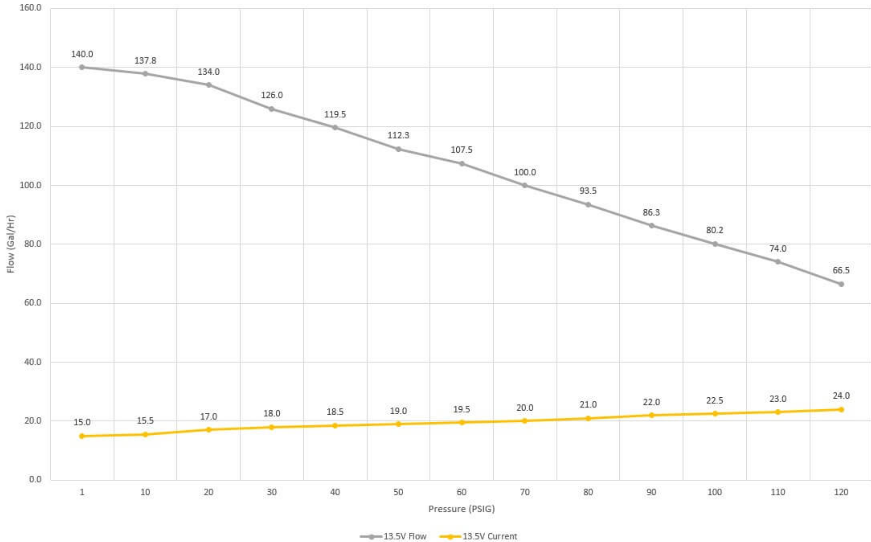
Single 525 LPH Flow Chart
