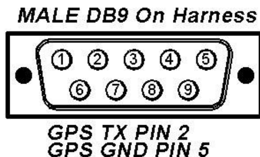
Figure 5. Typical GPS Connection
