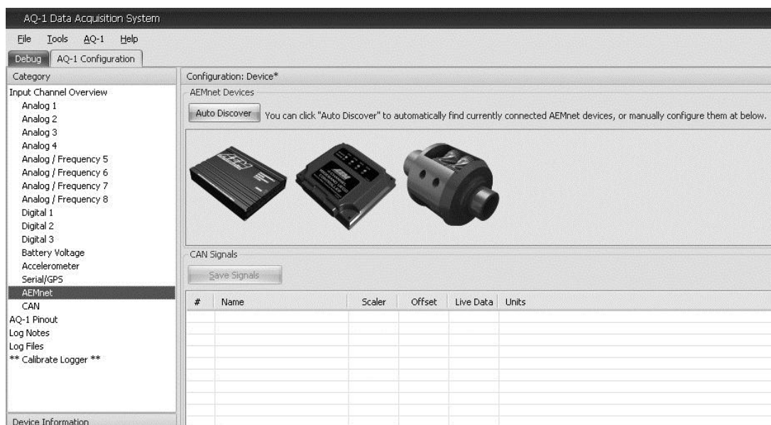
Figure 18. AEMnet Page
