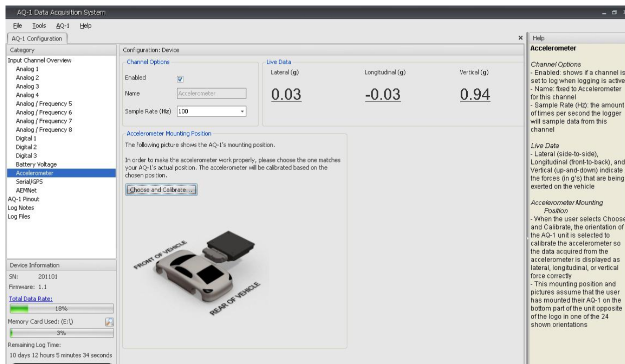
Figure 16. Accelerometer Page
