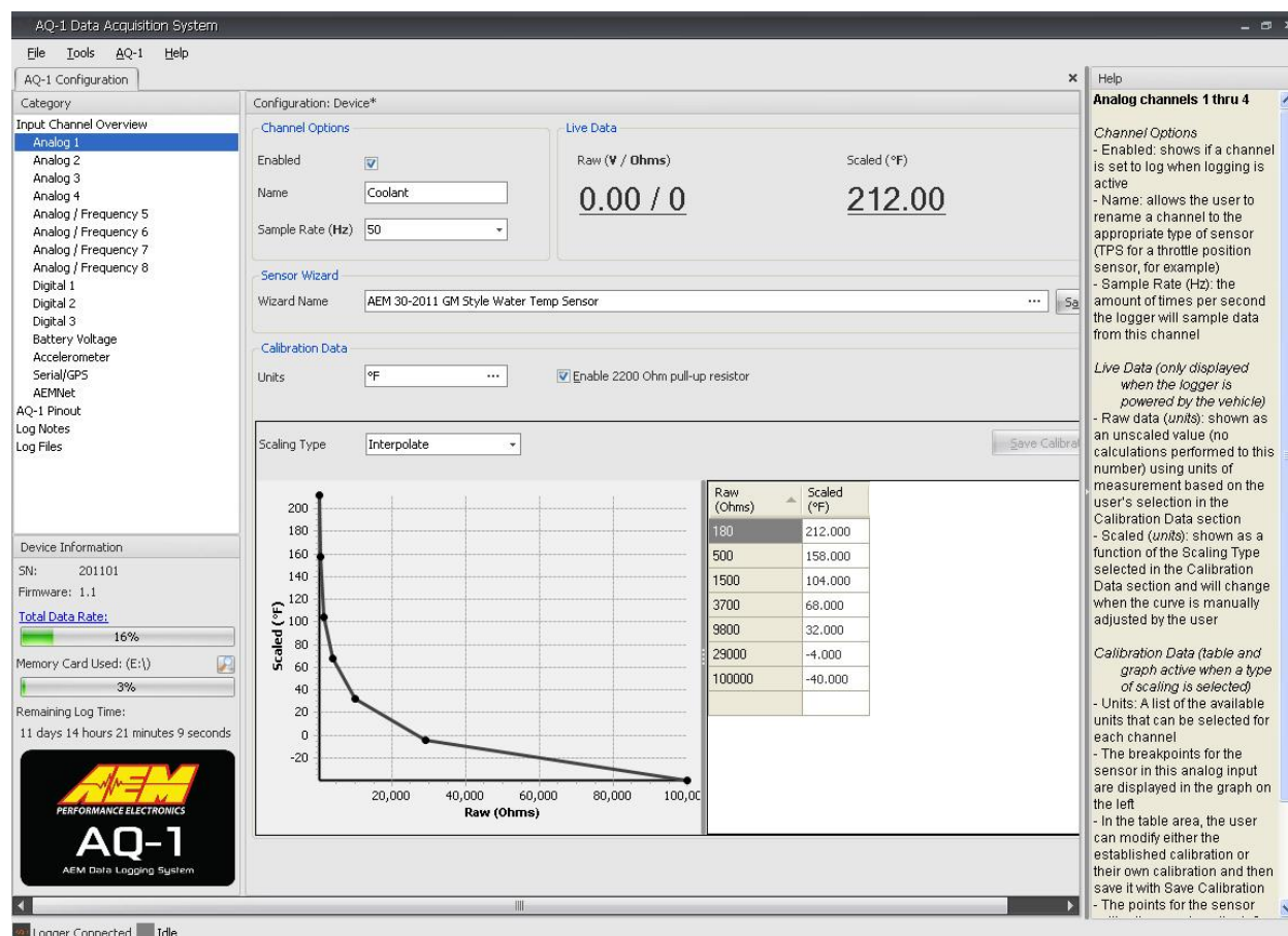
Figure 11. Analog 1 Configured for GM Style Water Temp Sensor
