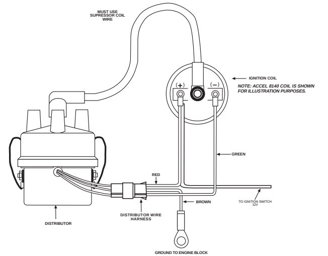
FIGURE 4 ACCEL POINTS ELIMINATOR WIRING DIAGRAM USING OEM PRIMARY RESISTANCE WIRE
