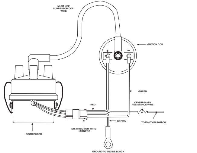
FIGURE 5 ACCEL POINTS ELIMINATOR WIRING DIAGRAM USING BALLAST RESISTOR
