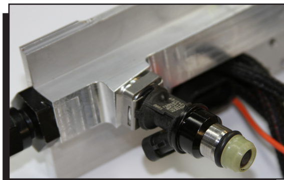
Figure 6 Injector Clips.
