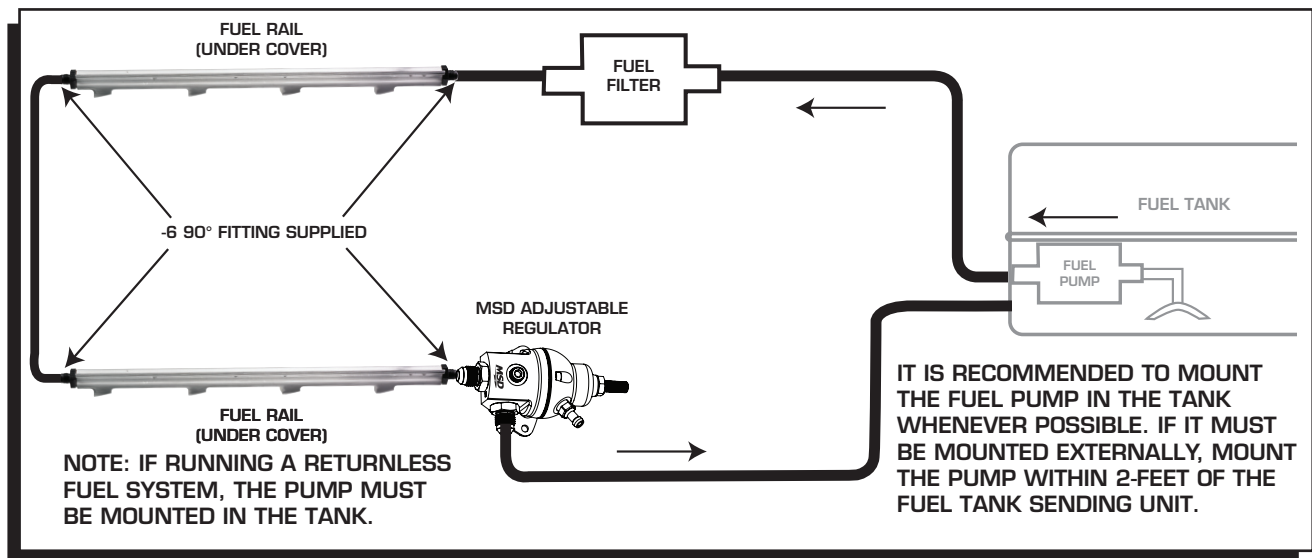
Figure 22 Fuel Line Routing.
