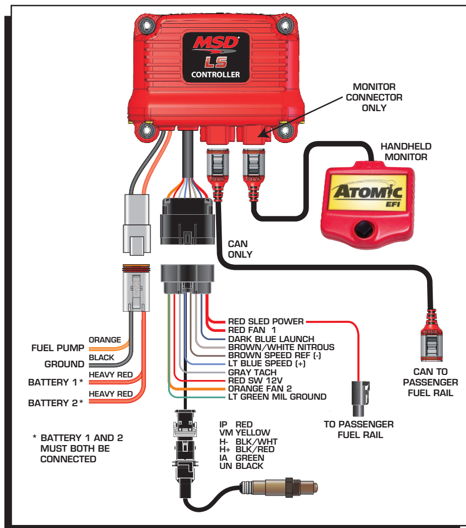
Figure 21 Power Module Wiring Diagram.
