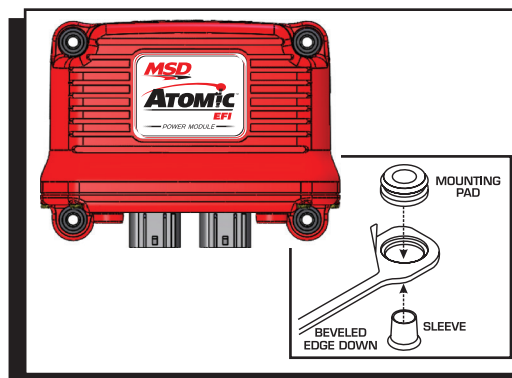
Figure 20 Mounting Hardware.
