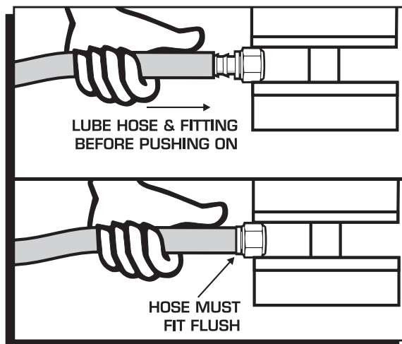
Figure 24 Installing Fuel Hose to the Push-Lock Fittings.
