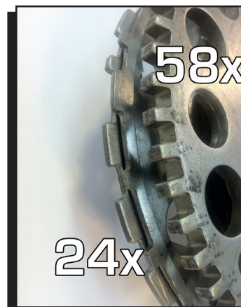
Figure 16 Crank Shaft Reluctors.
