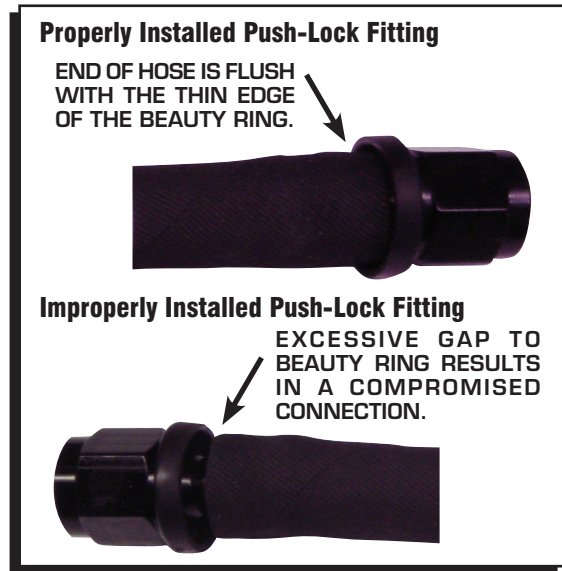
Figure 26 Installed Push-Lock Fitting.
