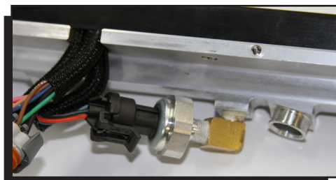
Figure 9 Fuel Pressure Sensor.
