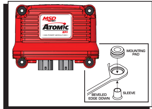
Figure 20 Mounting Hardware.
