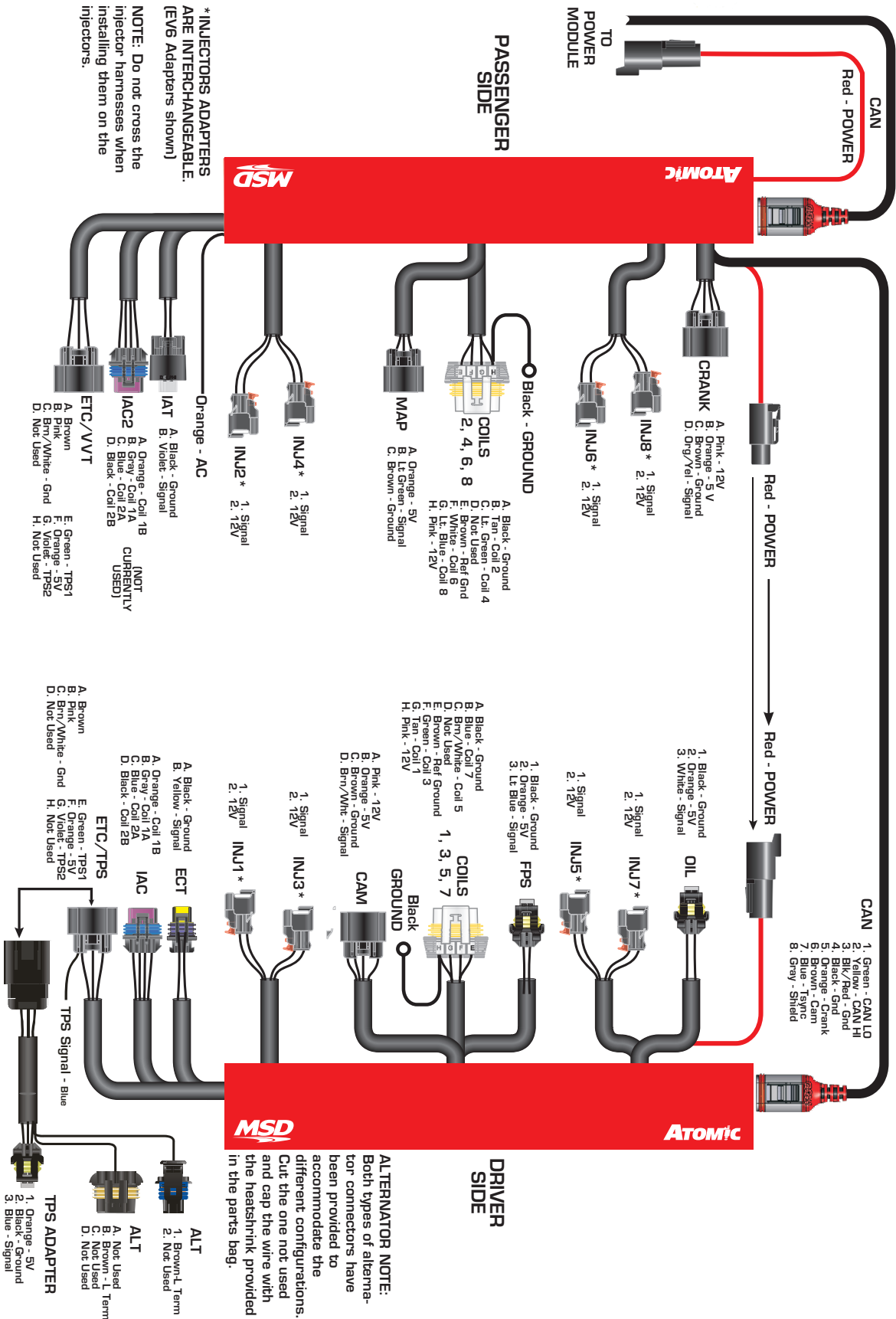
Figure 19 Wiring
