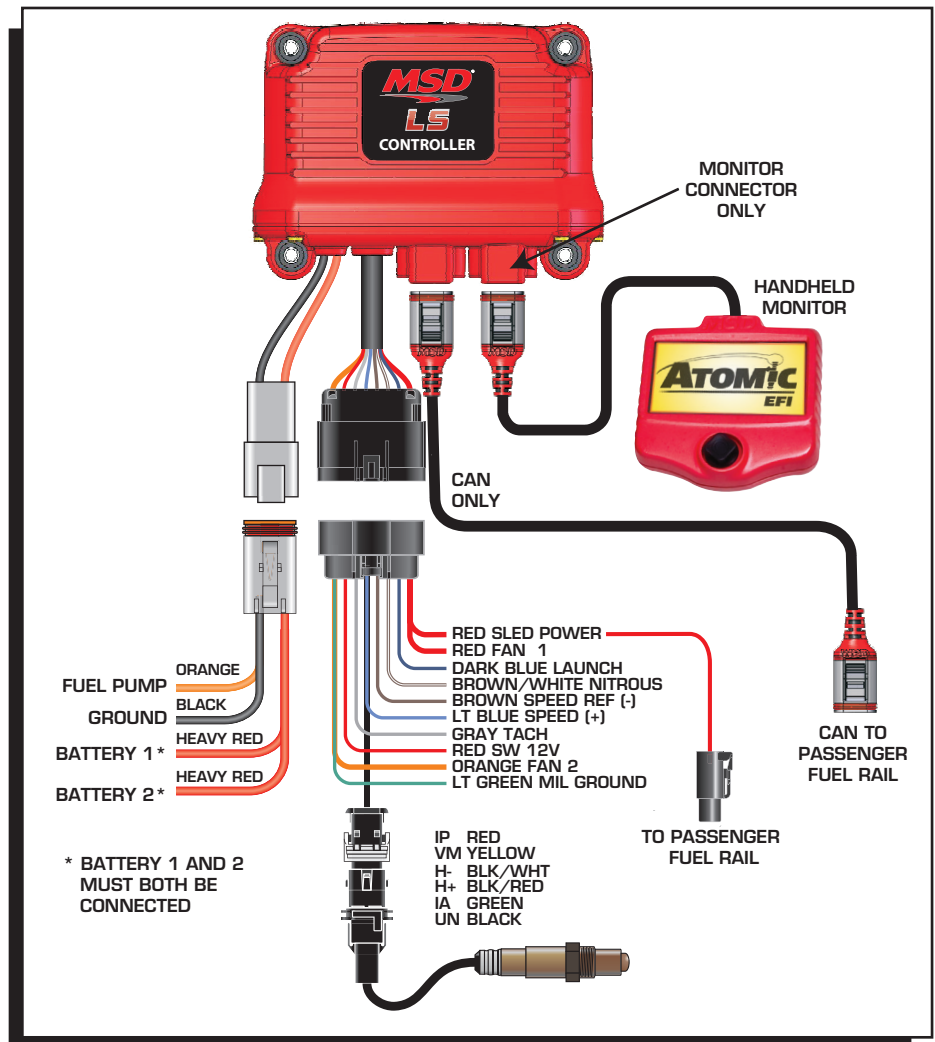
Figure 21 Power Module Wiring Diagram.
