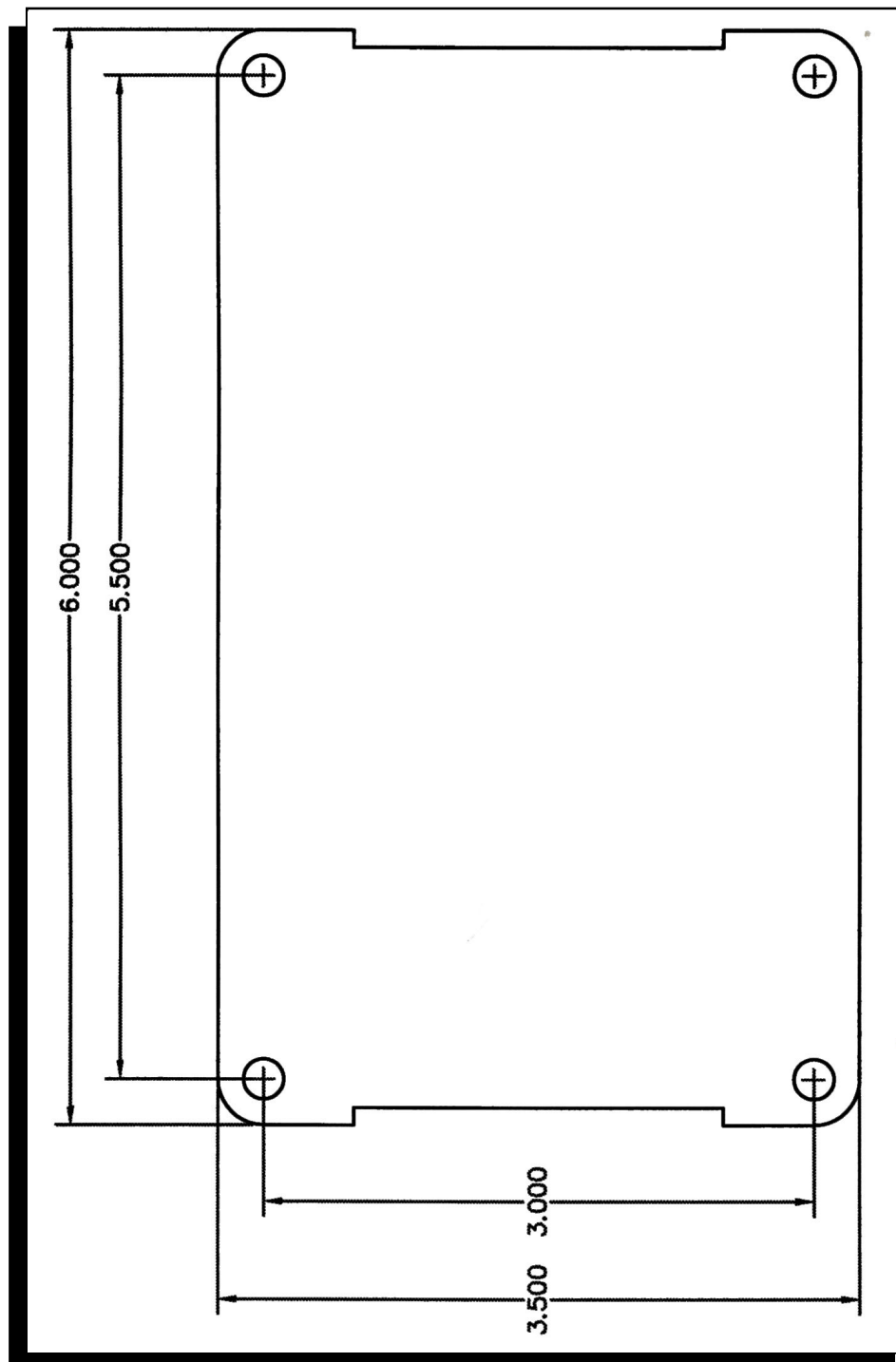
Figure 5 Mounting Template.
