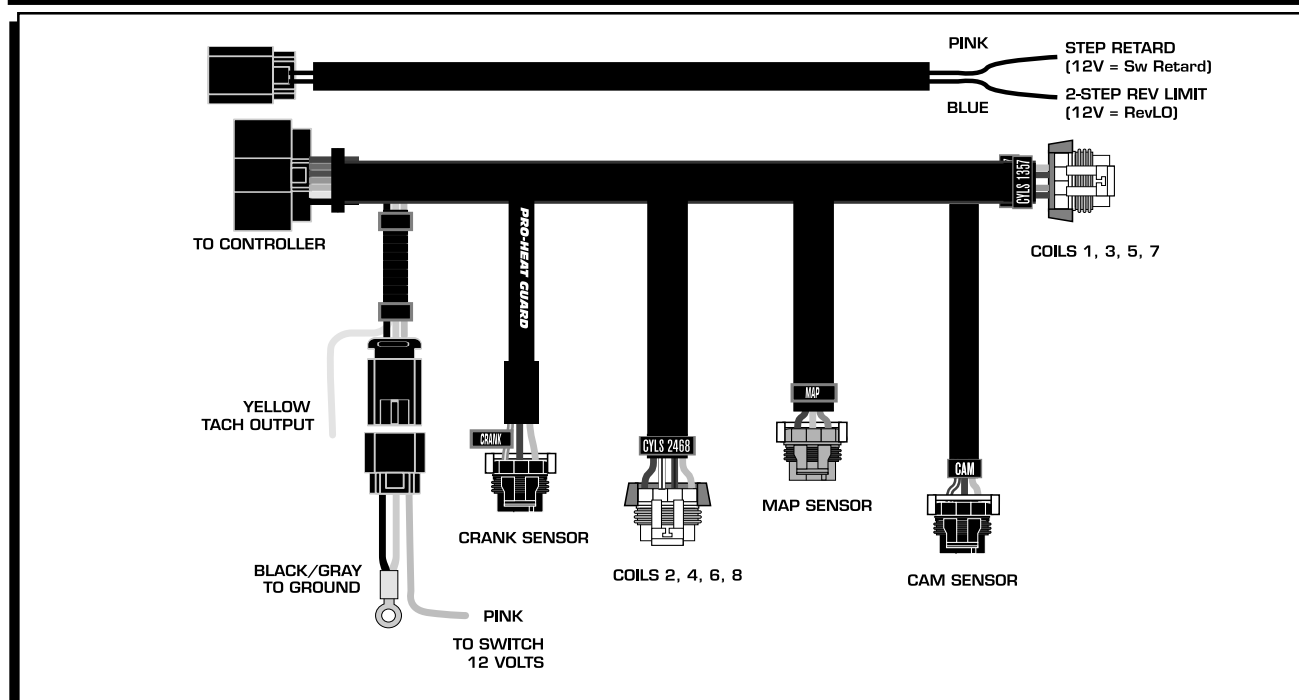
Figure 1 Wiring the MSD Gen III Controller.
