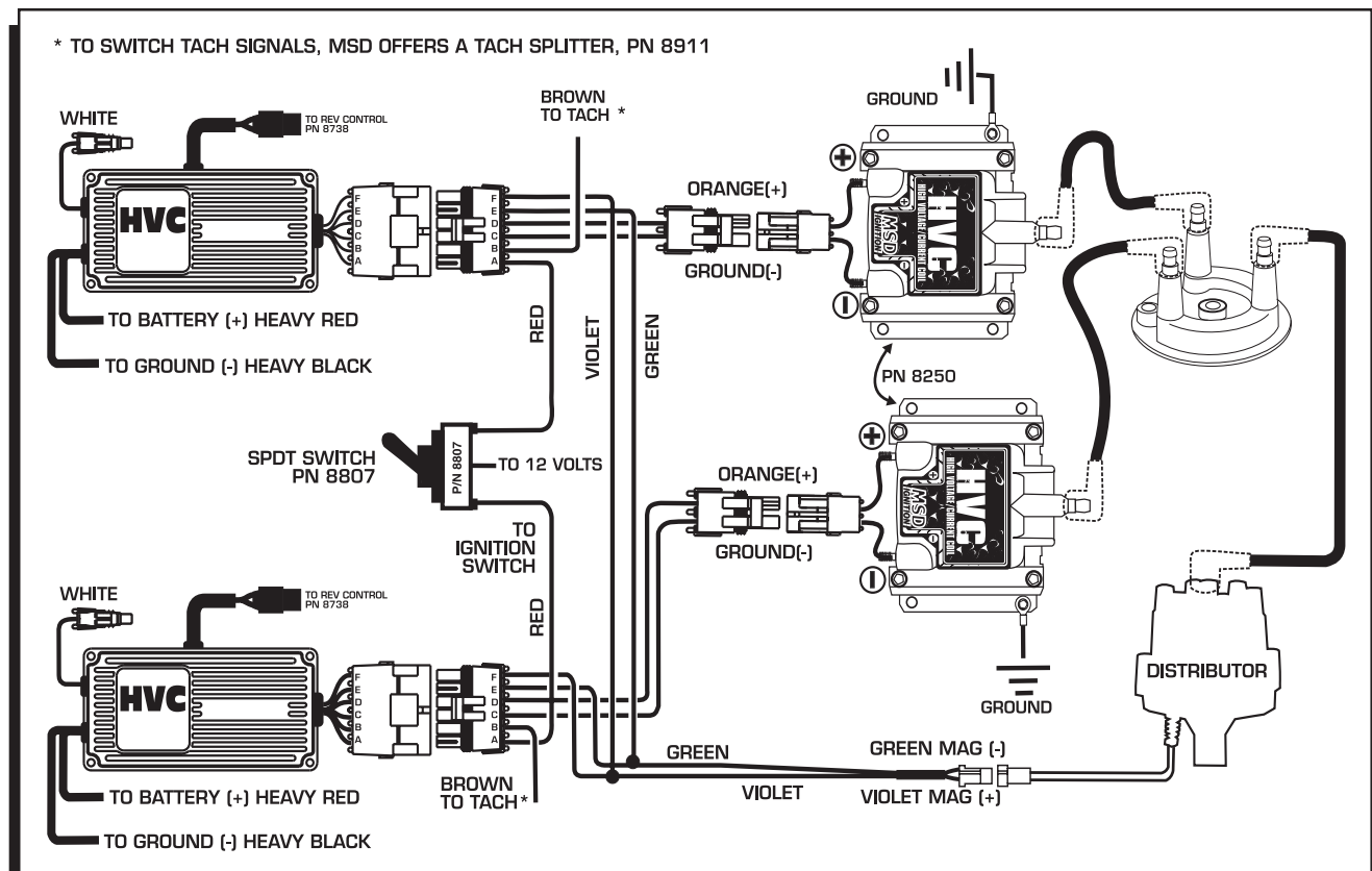
Figure 5 Dual Ignitions and Coils with a Single Pickup Distributor.
