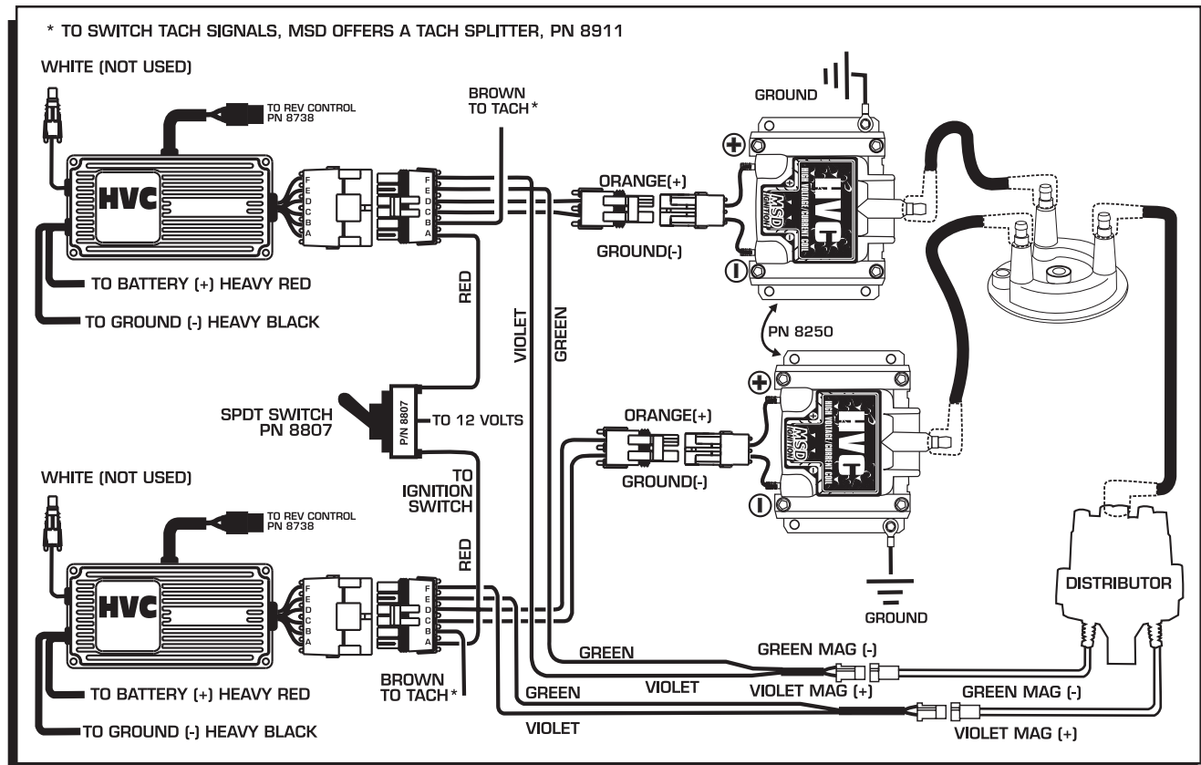
Figure 4 Dual Ignitions and Coils with a Dual Pickup Distributor.
