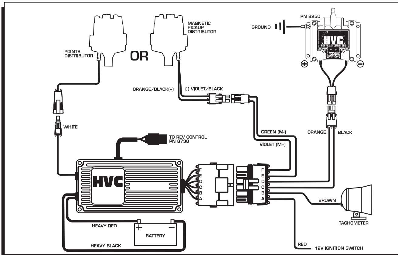
Figure 2 General Installation.
