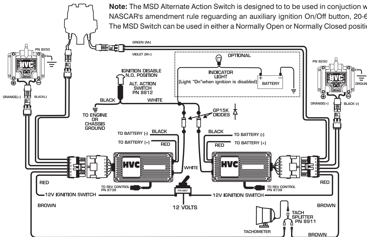
Figure 6 Complete Wiring with Tach Splitter and Alternate Action Switch.
