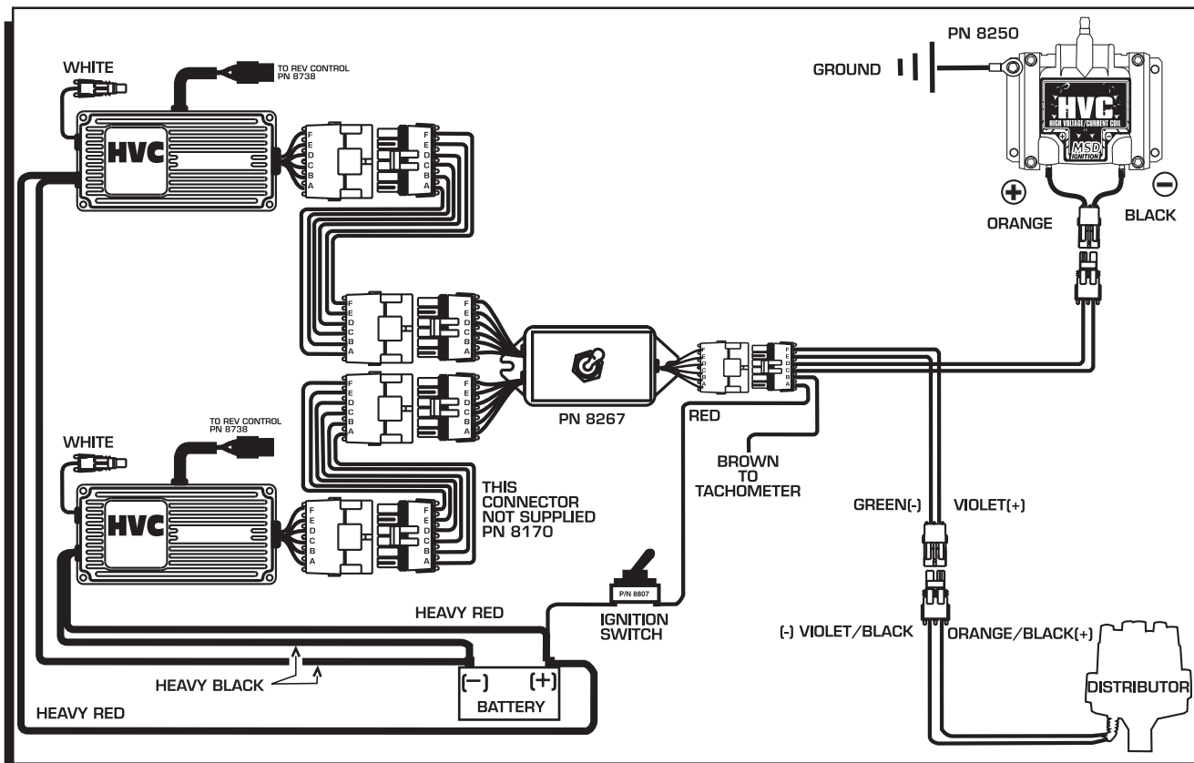
Figure 3 Dual Ignitions, Single Coil and Pickup Distributor.
