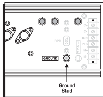
Figure 2 Ground Stud.
