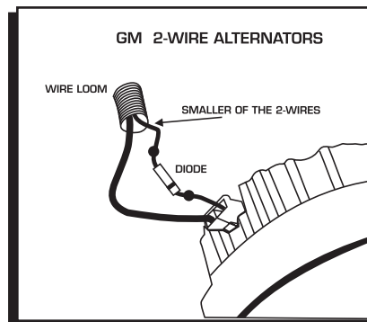
Figure 10 Installing the Diode to a 1973-1983 GM Vehicle.
