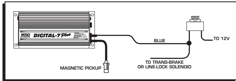
Figure 5 Wiring the 2-Step Rev Limit.
