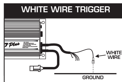
Figure 11 Checking for Spark with the white wire.
