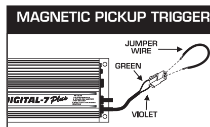
Figure 12 Checking for Spark with the Mag Pickup.
