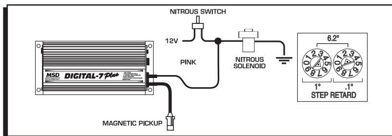
Figure 6 Wiring the Retard Stage.
