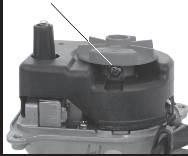
Figure 3 Replacing the Rotor.
