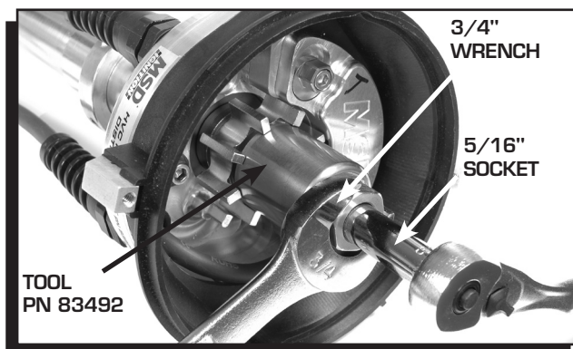
Figure 1 Removing the Reluctor.
