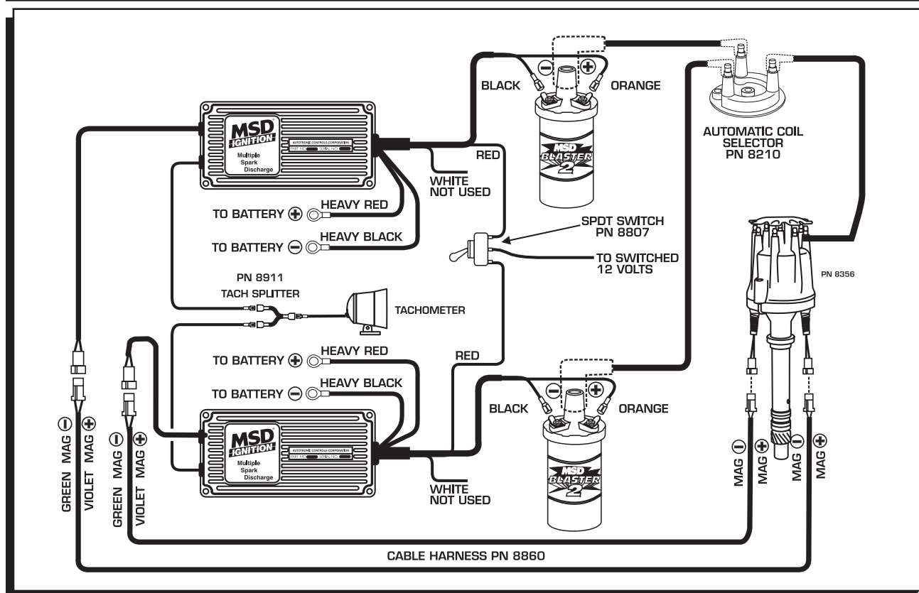
Figure 2 Wiring with MSD 6A Series Ignition Controls.
