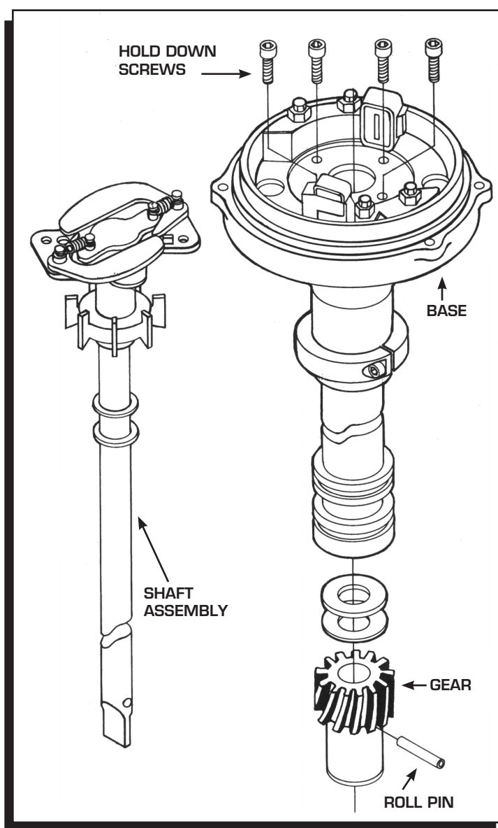
Figure 1 Disassembly.
