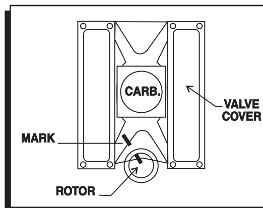
Figure 1 Marking the Position of the Rotor Tip.
