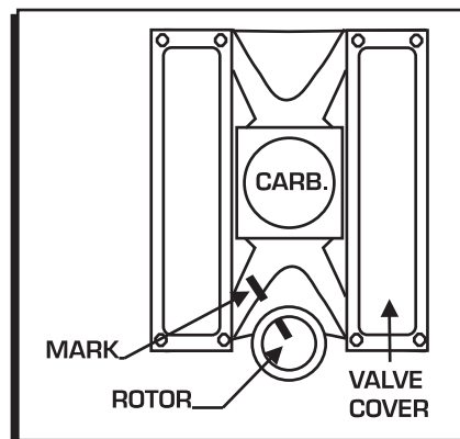
Figure 1 Marking the Rotor Location.
