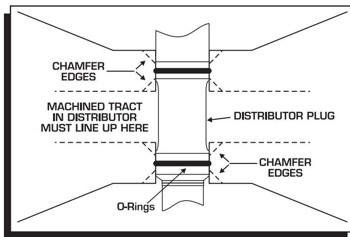
Figure 1 Alignment Of The Distributor Plug.
