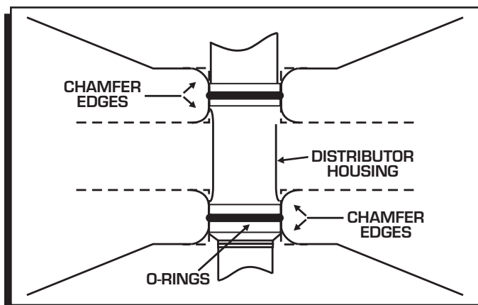
Figure 9 Modified Chevy Block for use with O-Rings.
