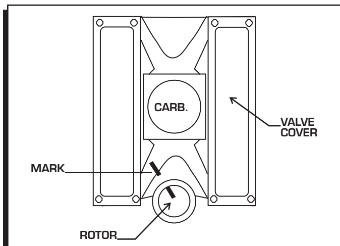
Figure 8 Marking the Rotor Location.
