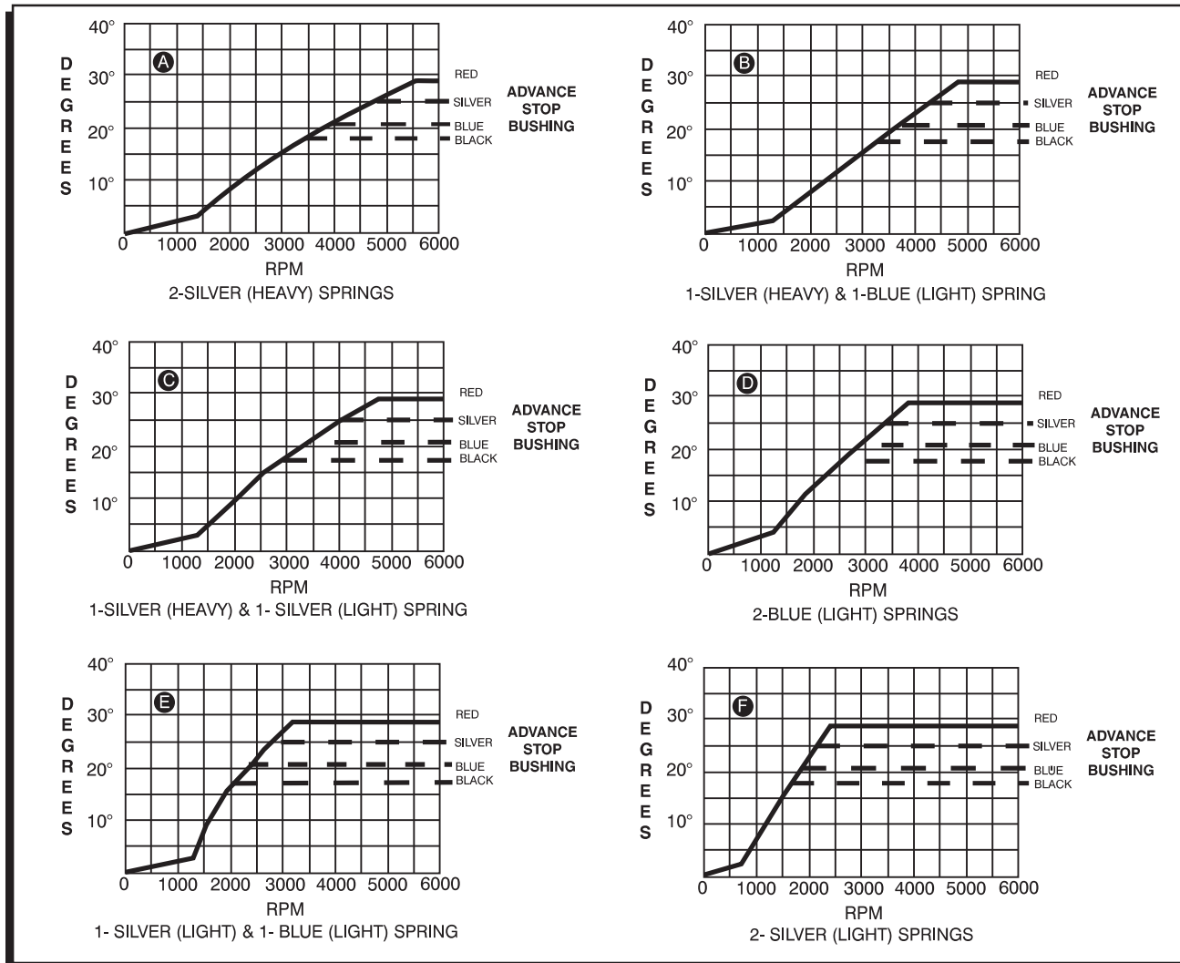
Figure 3 Advance Curves.
