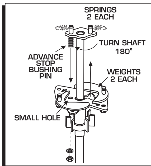
Figure 6 Locking Out the Centrifugal Advance.
