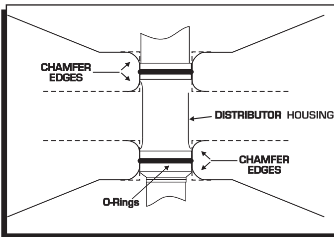
Figure 10 Modified Chevy Block for use with O-Rings.
