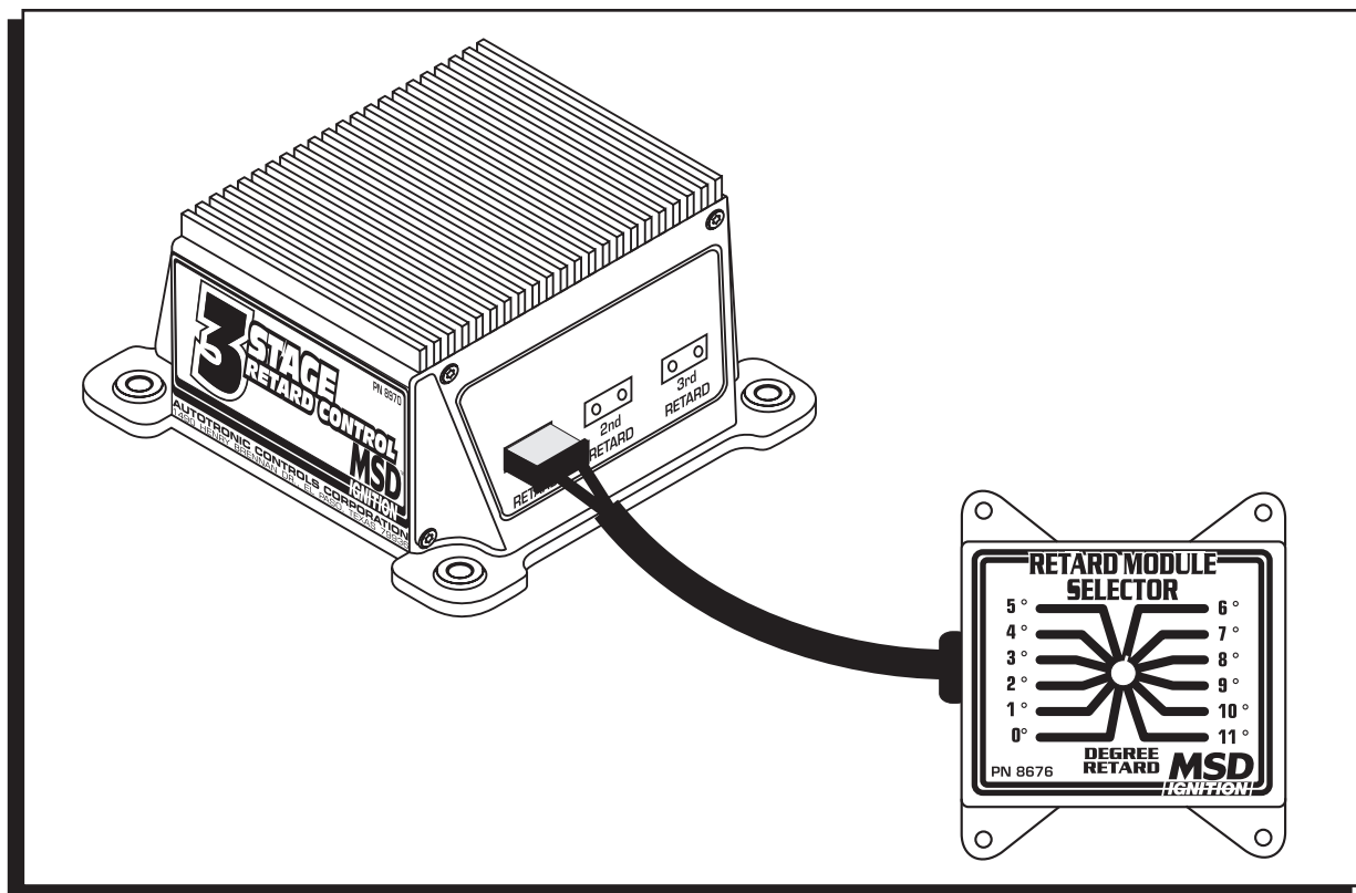
Figure 1 Retard Degree Module Selector Installation.
