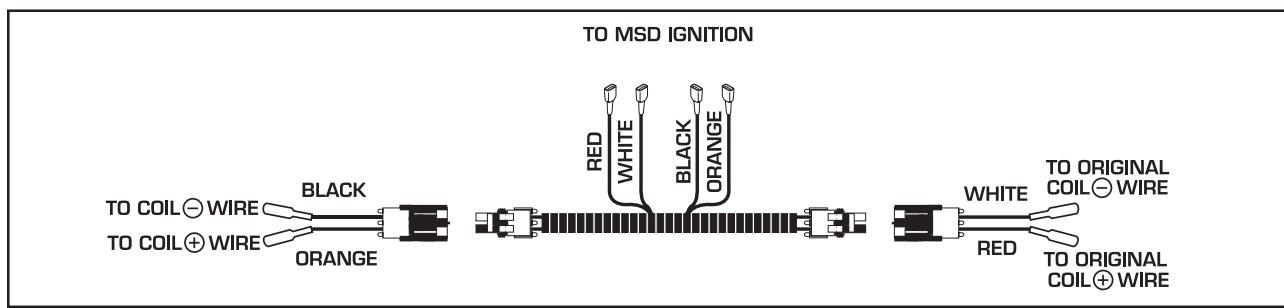
Figure 1 Wire Functions and Connections.
