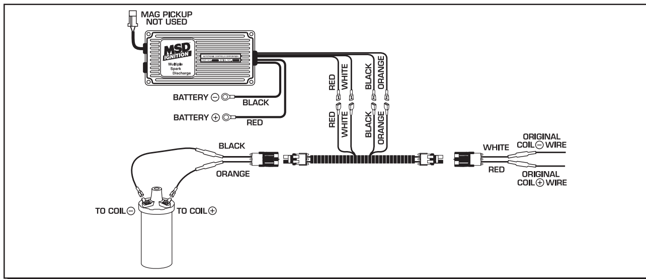
Figure 2 General Installation.
