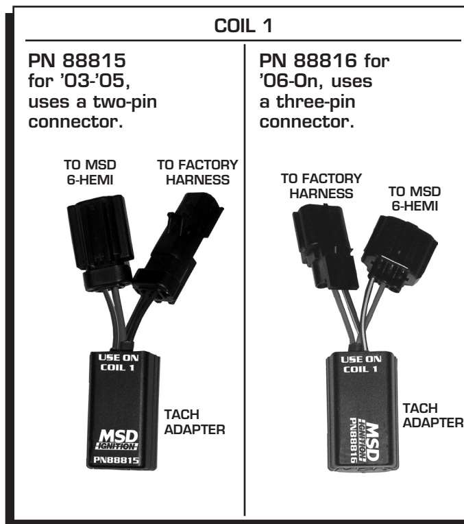
Figure 1 Coil 1 Tach Adapters.
