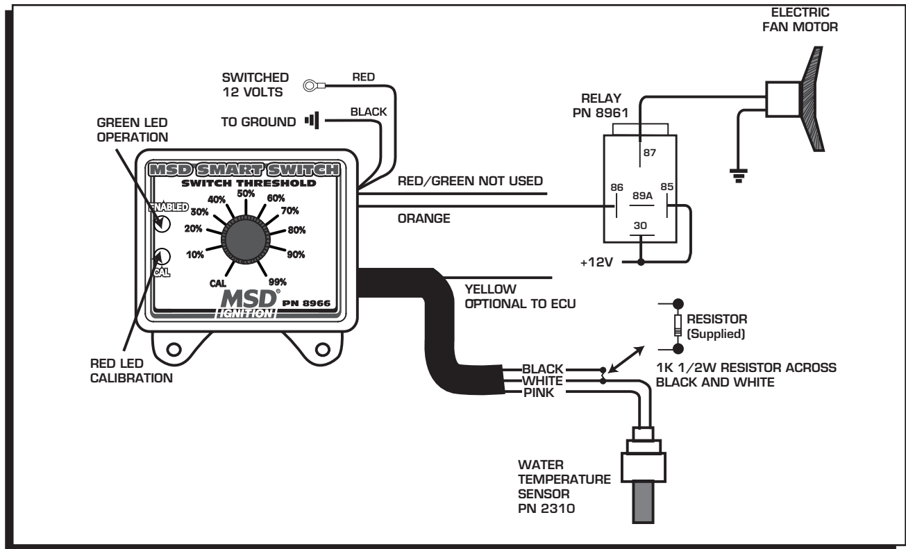
Figure 3 Wiring to Activate a Cooling Fan.
