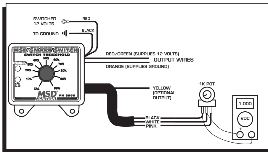
Figure 2 Potentiometer Calibration
