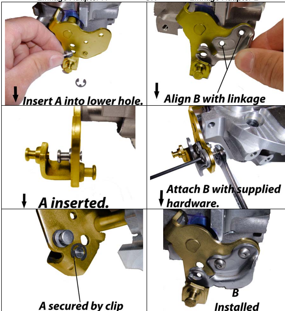
Linkage Adapter A
