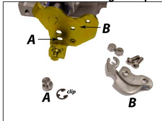
Linkage Adapter A
