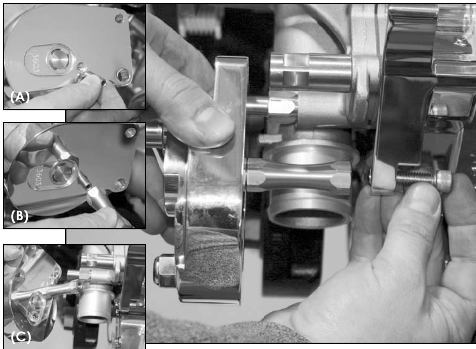
Figure 13: Install Tensioner
