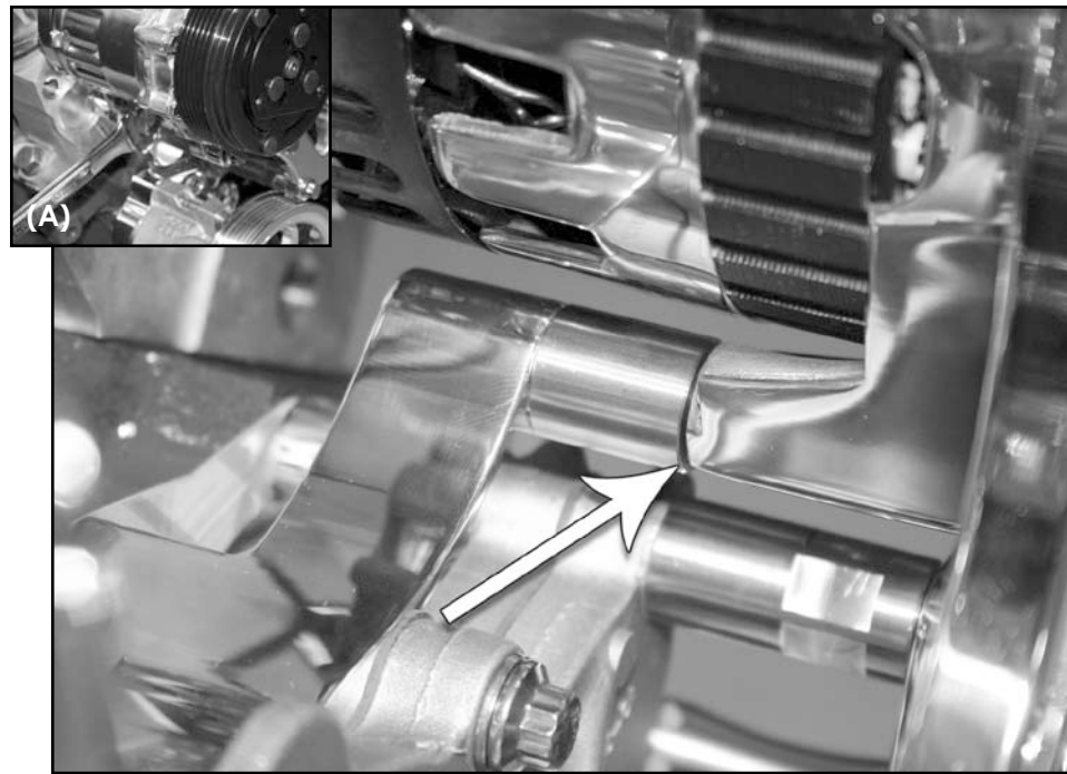
Figure 18: Complete Bridge Bracket Installation
