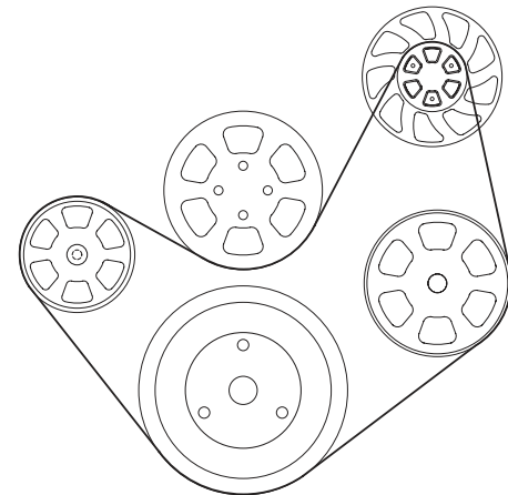
Illustration: Serpentine Belt Path with Power Steering
