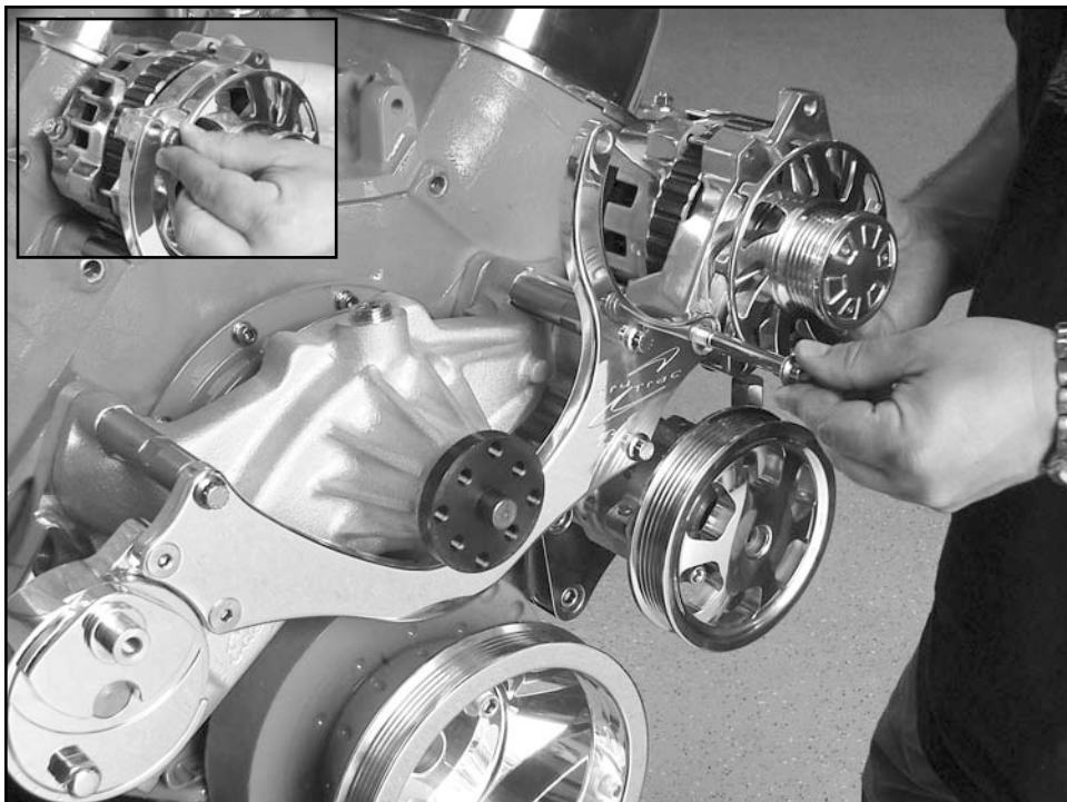
Figure 11: Attaching Alternator
