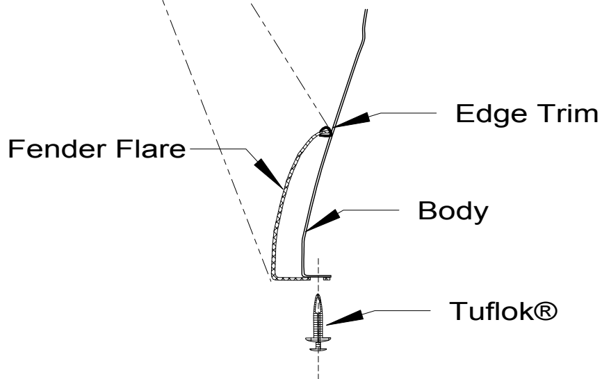
Illustration #3 Cross Section
