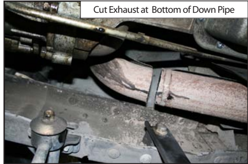
Cut Exhaust at Bottom of Down Pipe
