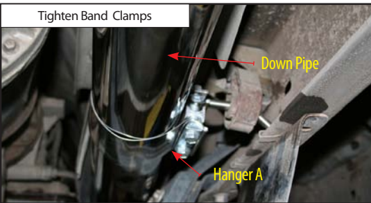
Complete System Installed
