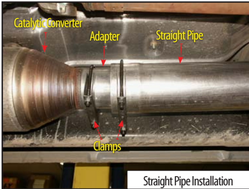
Measure for Straight Pipe
