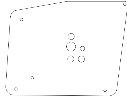
Firewall Block Off PN#10-1033-2
