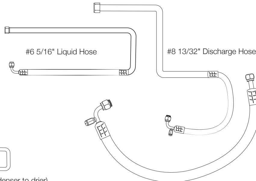
#10 1/2" Suction Hose
