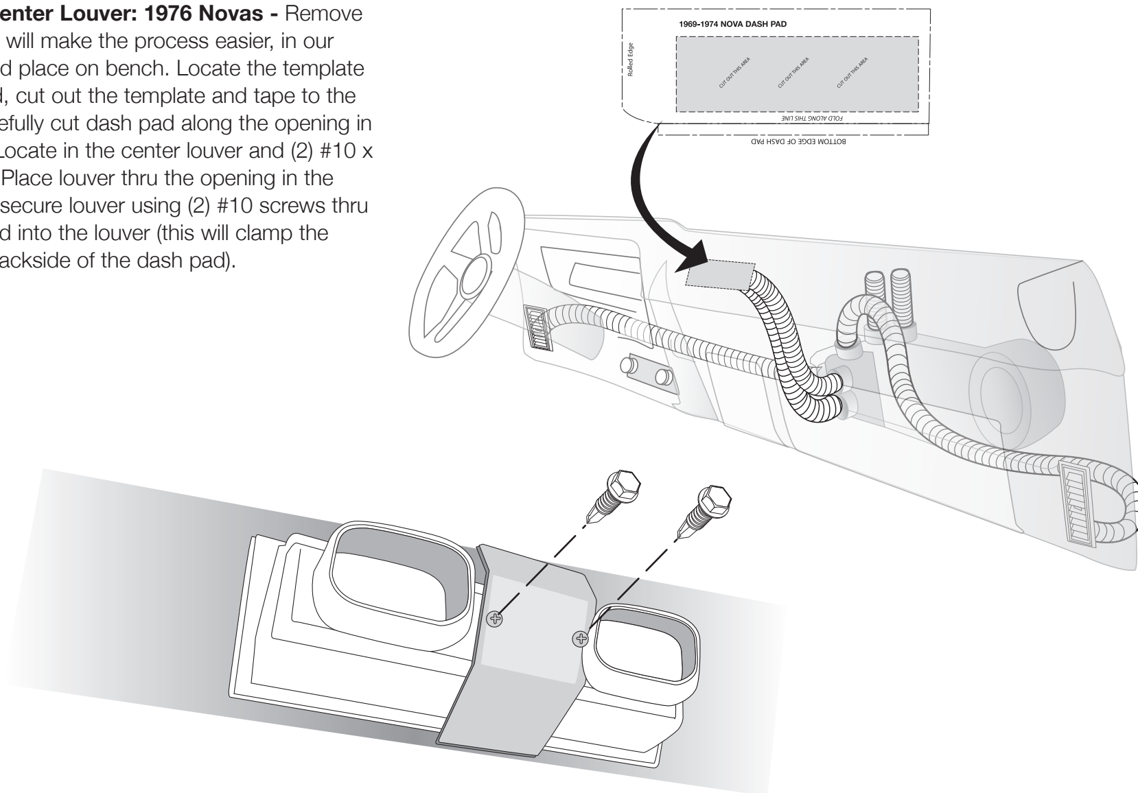
VIEW FROM BACK SIDE OF VENT ASSEMBLY, BEHIND THE DASH PAD
