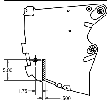
UNDERBODY PANEL TRIM DIAGRAM FOR SEDAN
