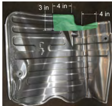
HEAT SHIELD TRIMMING DIAGRAM
