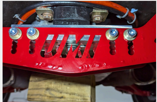
Figure 5: Adjustment Block Installed
