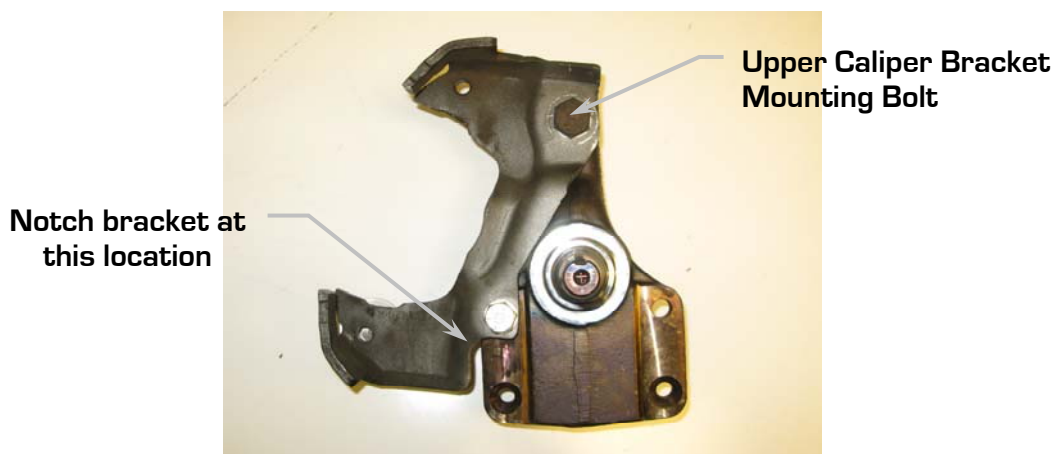
Figure 2 - Notching Stock Caliper Bracket
