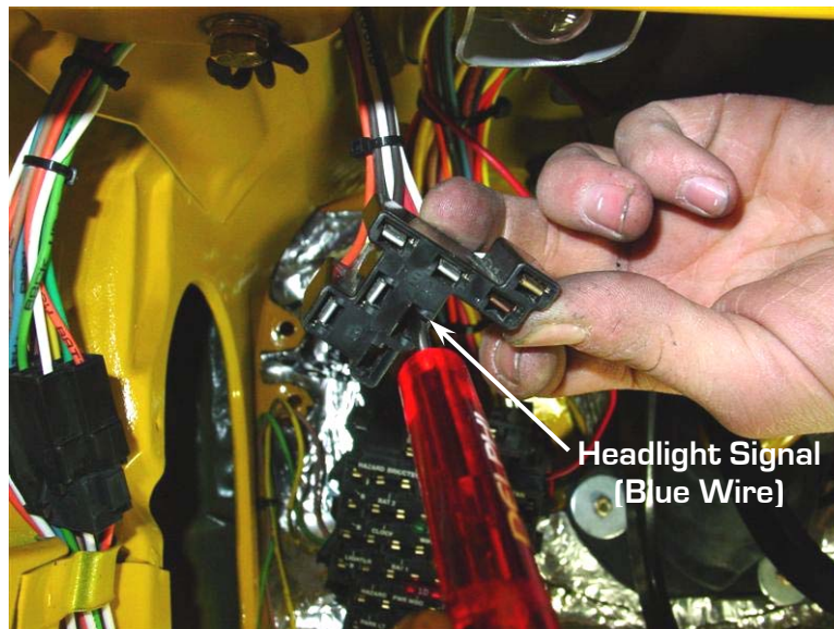
Figure 6 – Locating the Blue Wire
