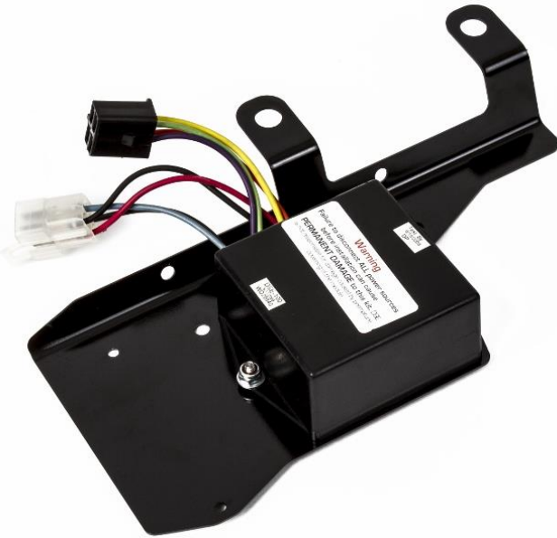
Figure 35 – Headlight Module
