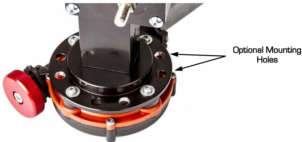
Figure 15 - Motor Orientation
