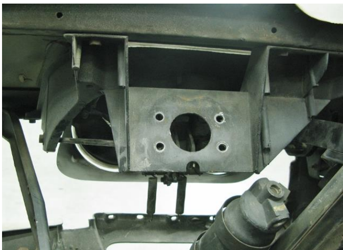
Figure 14 - Install Actuator Assembly
