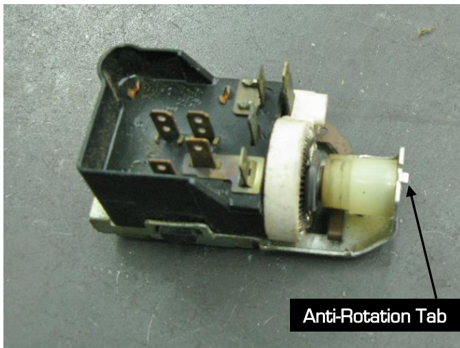
Figure 40 – Install Headlight Switch
