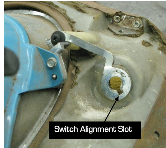
Figure 40 – Install Headlight Switch
