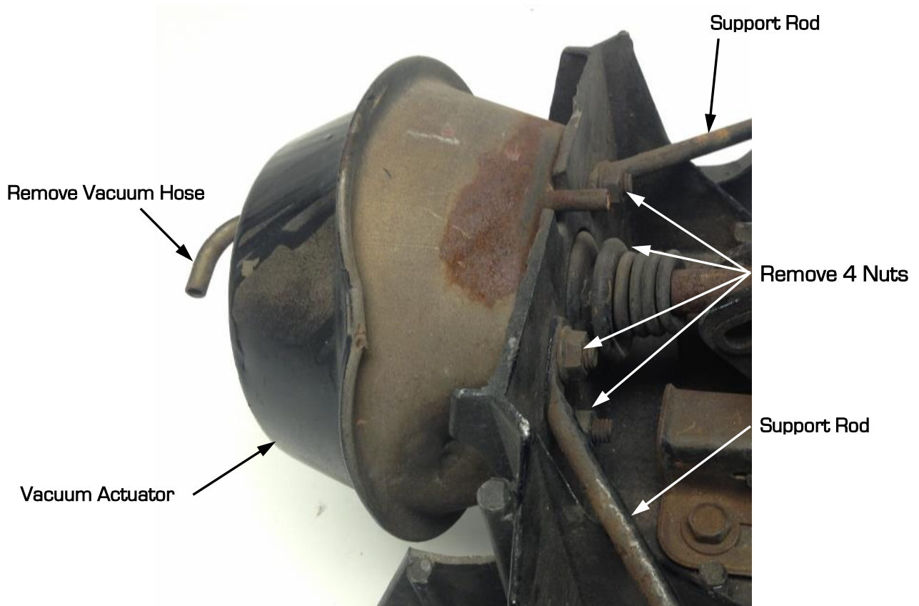
Figure 5 - Remove Vacuum Actuator
